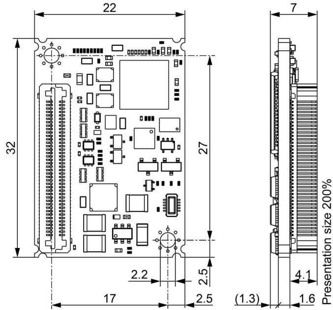
Figure 2-4 EPOS4 Micro 24/1.5 CAN – Dimensional drawing [mm]
