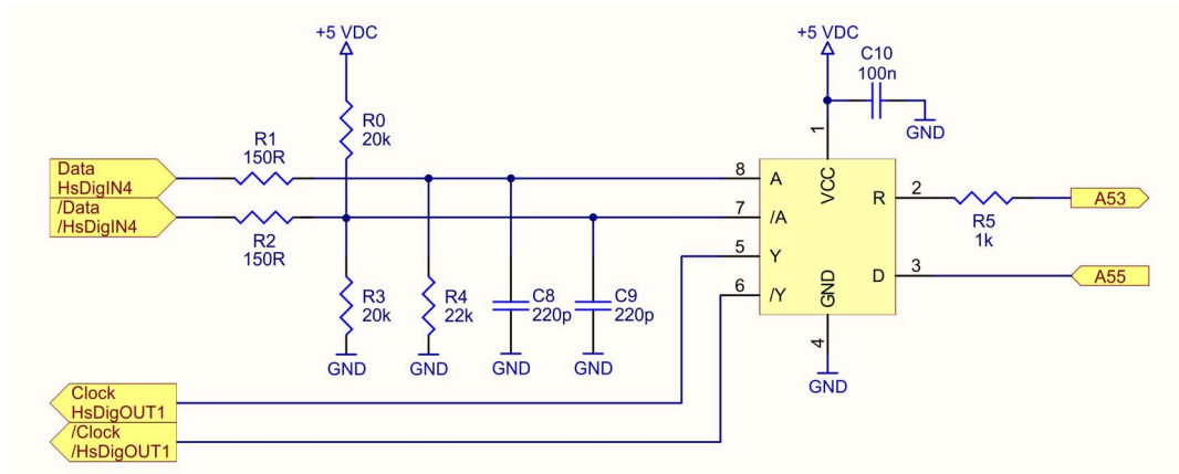
Figure 4-43 Wiring of RS422 transceiver
