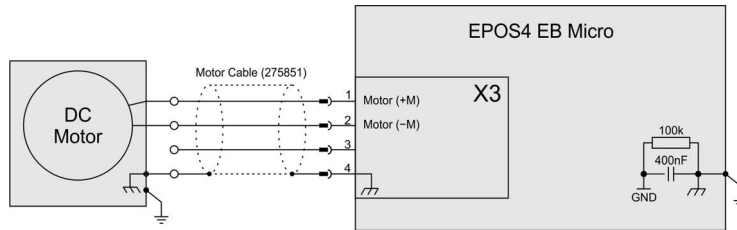
Figure 5-52 DC motor
