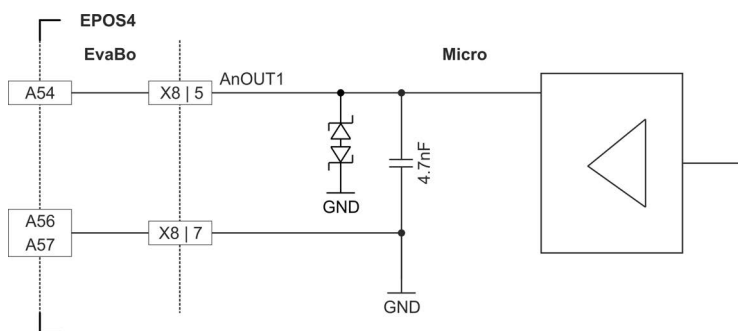
Figure 3-36 AnOUT1 circuit
