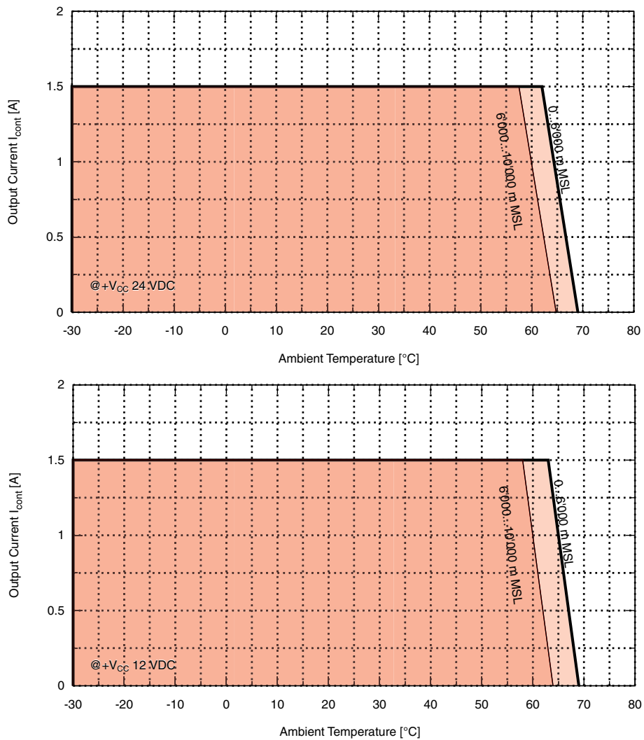
Figure 2-2 Derating of output current
