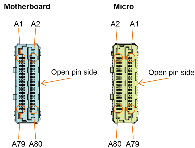
Figure 4-47 EPOS4 Micro 24/1.5 CAN – Terminal/socket placement (mating)
